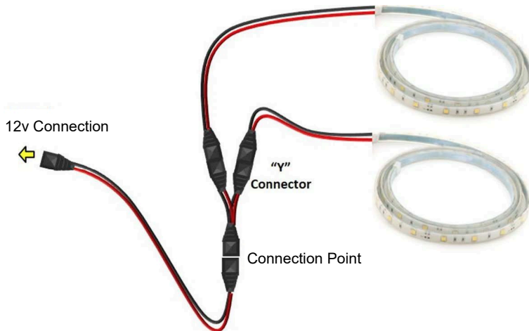
Y-Connector used in a two light application without a remote transmitter.
