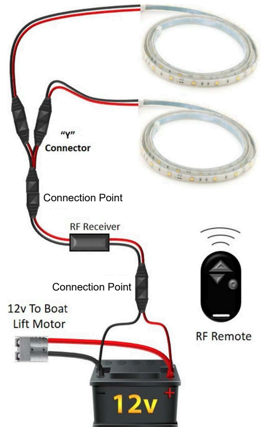
Y-Connector used in a two light application with a remote transmitter.
